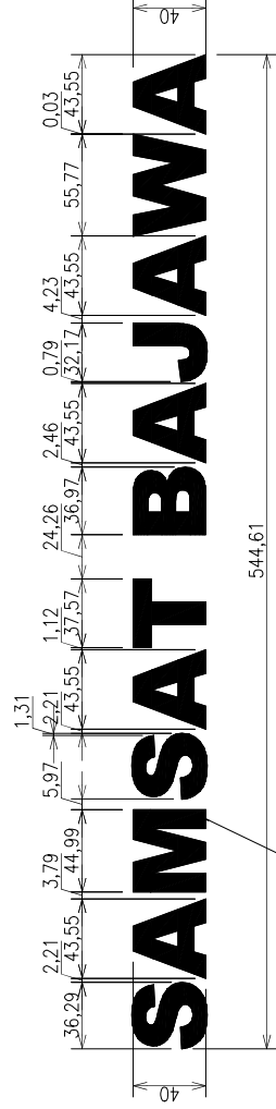
DETAIL HURUF TIMBUL
